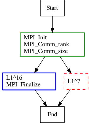
Figure 6: dlBug
